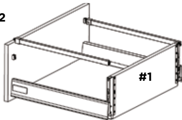
FIG. 20 Keep the drawer open. Fit, push down and click the rear of the top side bars into position.
